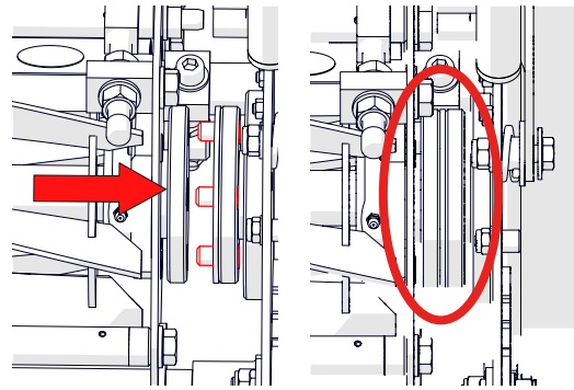
Fig.7E - Lower the new cassette in and slide across, engaging with three pins.
