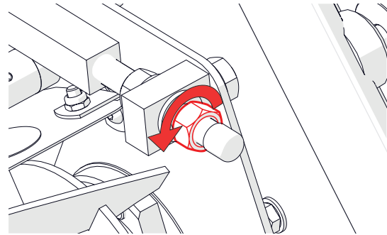
Fig.11C - Loosen the lock nut
