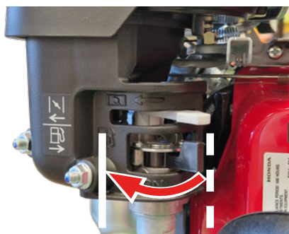
Fig.13C - Set the fuel lever to closed position.
