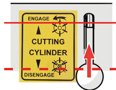
Fig.15B - Engage the cassette lever.
