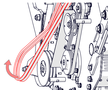
Fig. 18C - Remove and replace the belt.
