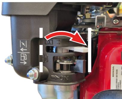
Fig.12H - Move choke lever into open position.
