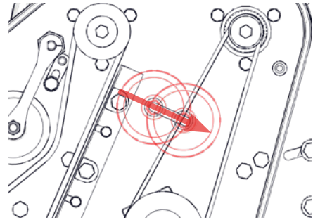
Fig. 16J - Adjust the pulley to add pressure to the belt.
