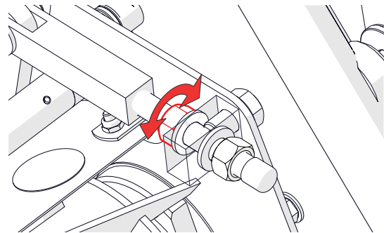
Fig.11D - Tighten/loosen the adjustment nut
