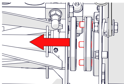
Fig.7C - Slide cassette until pins are visible
