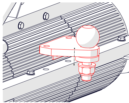
Fig. 28A - Position the towball bracket.
