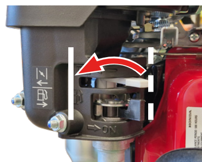
Fig.12D - Choke lever closed.
