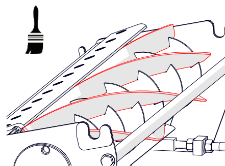
Fig.19A - Apply paste to the blades
