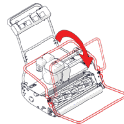
Fig.2A - Lower grass box frame.
