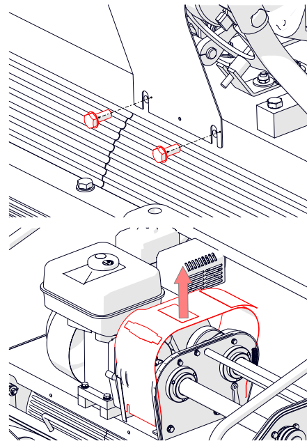
Fig.17A - Transmission guard removal.
