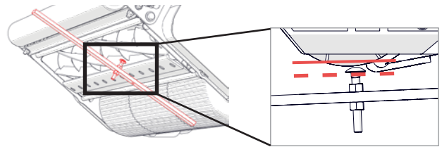
Fig.8D - Position the setting bar and observe distance between the top of the shear blade and bottom on the bolt head. In this example, the bolt head is below the shear blade, indicating the machine cut height is currently too high and therefore needs lowering.
