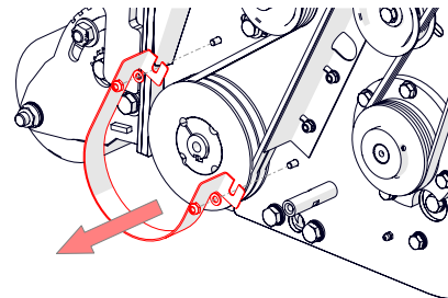
Fig. 18B - Remove the belt guide.
