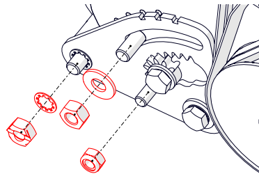
Fig. 27A - Remove the three fixings as illustrated.
