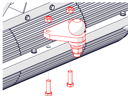
Fig. 28B - Insert the bolts from underneath and tighten.
