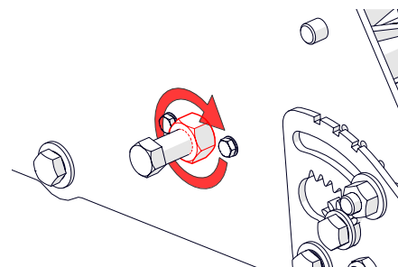
Fig.7G - Secure the locknut
