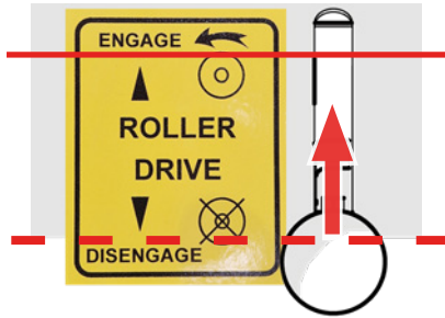
Fig.14B - Engage the drive lever.
