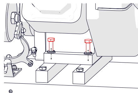
Fig.17B - Remove engine bolts from bearers.
