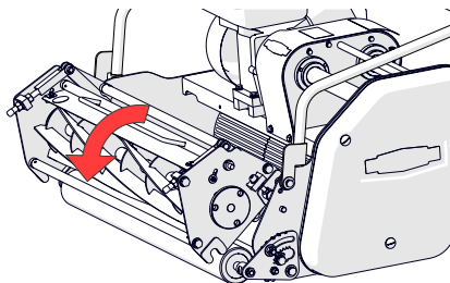
Fig.7C - Slide cassette until pins are visible
