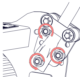
Fig.10B - Loosening the inner nut
