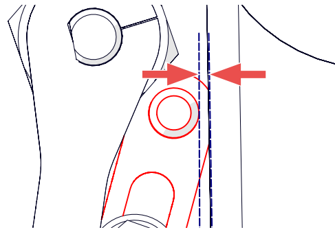
Fig.24B - Keep a very small gap between the peg and belt when pulley in the engaged
