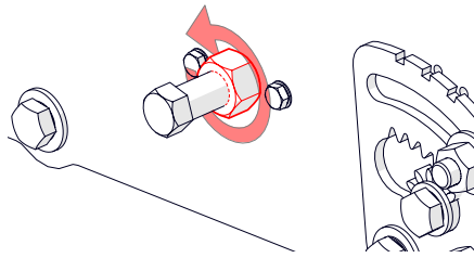
Fig.7A - Loosen retaining bolt locknut
