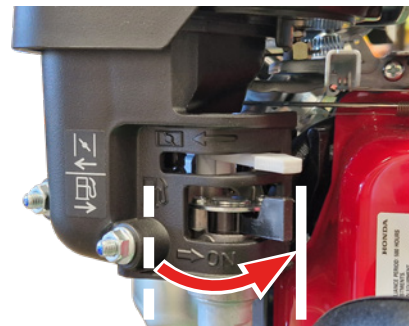
Fig.12C - Fuel lever open.
