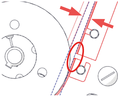
Fig. 16E - Ensure both belt guides are level (i.e.no step) (circled) and sufficient gap between the belt and belt guide (lines).
