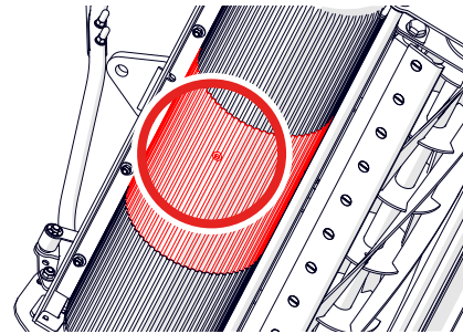
Fig.23B - Roller drain hole pointing downwards.
