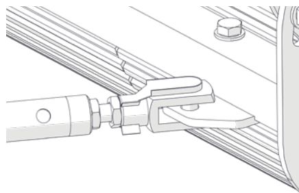
Fig. 28B - Insert the bolts from underneath and tighten.
