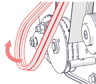
Fig. 16D - Remove and replace the belt.
