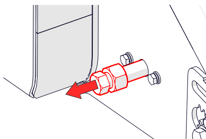
Fig. 8C - Unscrew retaining bolt
