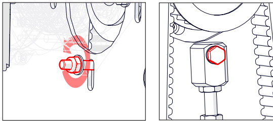
Fig. 18C - Loosen slightly the tensioner block/motor nut.
