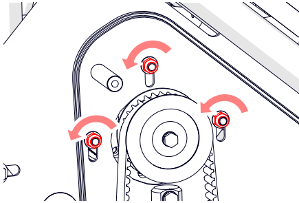
Fig. 18B - Loosen slightly the motor 3 x top nuts.
