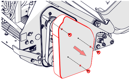
Fig. 18A - Remove 3 x outer screws and cover.
