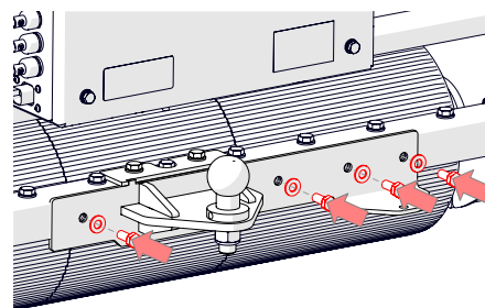
Fig. 26B - Insert the top bolts and tighten loosely.
