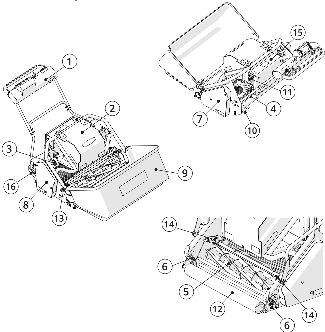
Fig.4. Machine components overview
