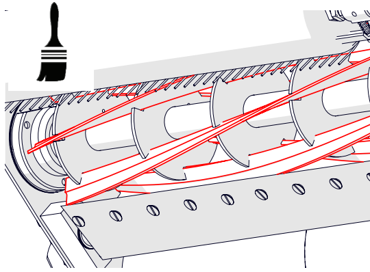
Fig.19. Backlapping
