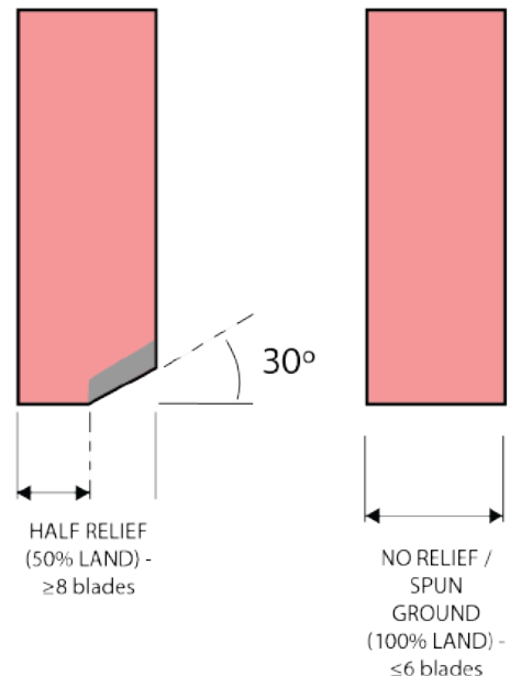
Fig.20. Recommended cylinder grind angle
