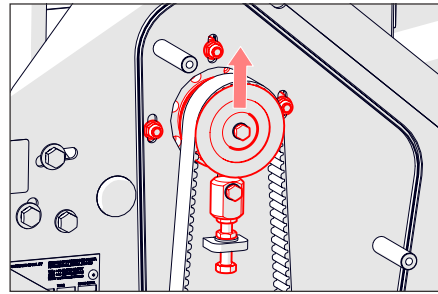
Fig. 18F - Replace the belt.
