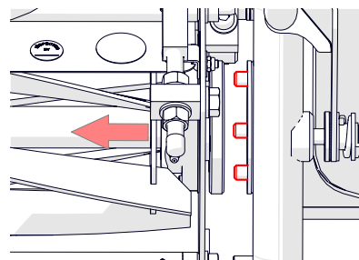
Fig. 8D - Slide cassette until pins are visible
