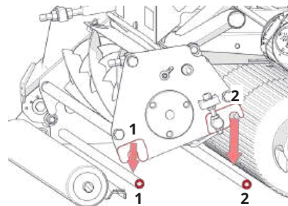
Fig. 8F - Lower cassette onto tie-bars (cut-through view for clarity).
