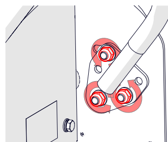
Fig. 11B - Loosening the inner nut
