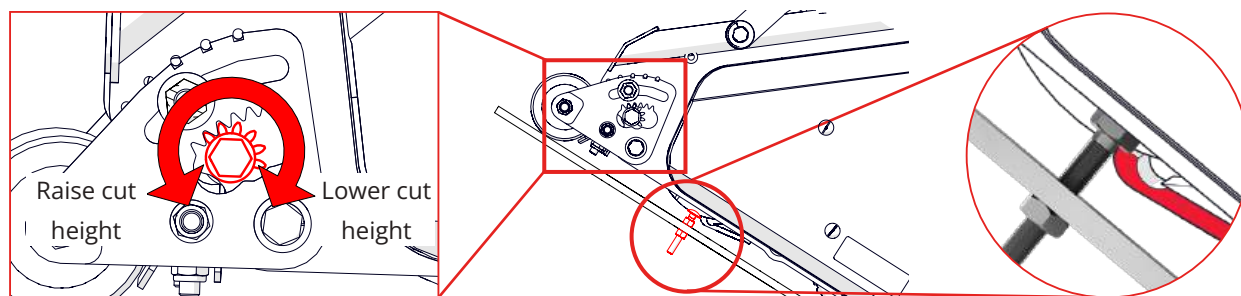
Fig. 9E - Rotate the toothed gear while offering up the setting bar. Stop when the head rests level/within the shear blade
