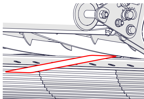
Fig. 12B - Repeating adjustment for other side
