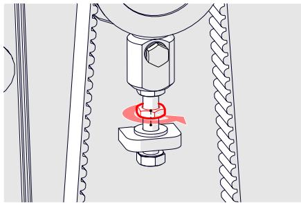
Fig. 18D - Loosen fully the tensioner block locking nut.
