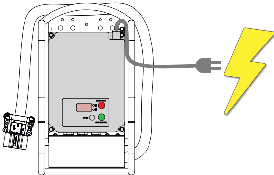
Fig. 17A - Plug the charger into the mains socket
