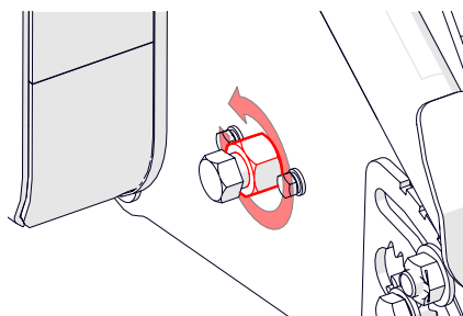
Fig. 8B - Loosen retaining bolt locknut
