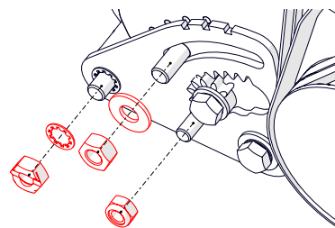
Fig. 25A - Remove the three fixings as illustrated.
