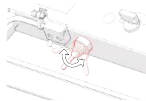
Fig. 15C - Power the cylinder unit on
