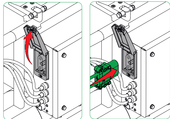
Fig. 17C - Remove the machine charging connector and plug into the charger
