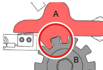
Fig. 23A - Brake hammer (A) engaging correctly with the cut-outs of the brake disc (B).
