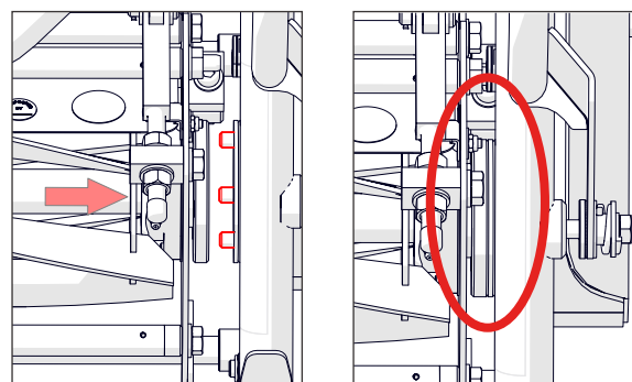
Fig. 8G - Lower the new cassette in and slide across, engaging with three pins.
