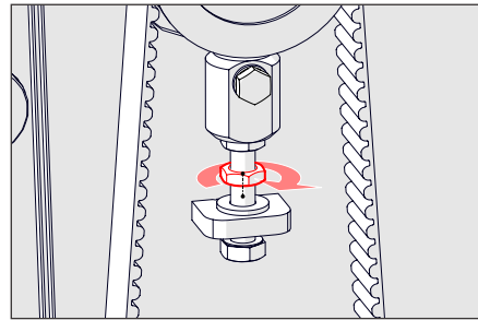
Fig. 18G - Tighten the belt and tensioner block locking nut.
