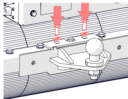
Fig. 26B - Insert the top bolts and tighten loosely.
