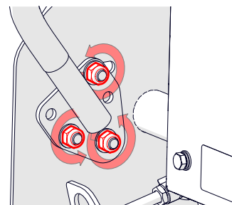
Fig. 11C - Repeating adjustment for other side
