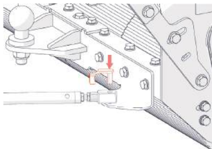
Fig. 26D - Secure steering cross-brace with clevis pin.
