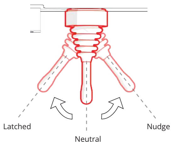
Fig. 6C - Drive Toggle Switch
