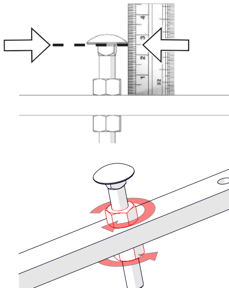
Fig. 9A - Adjust bolt to desired cut height and secure nuts (above example set for 25 mm)
