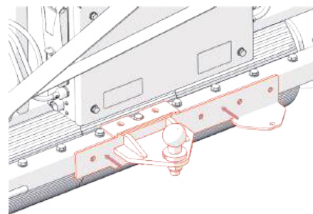
Fig. 26A - Position the towball bracket.
