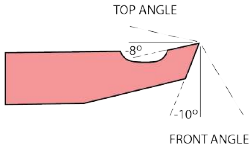
Fig.21. Recommended shear blade grind angle
