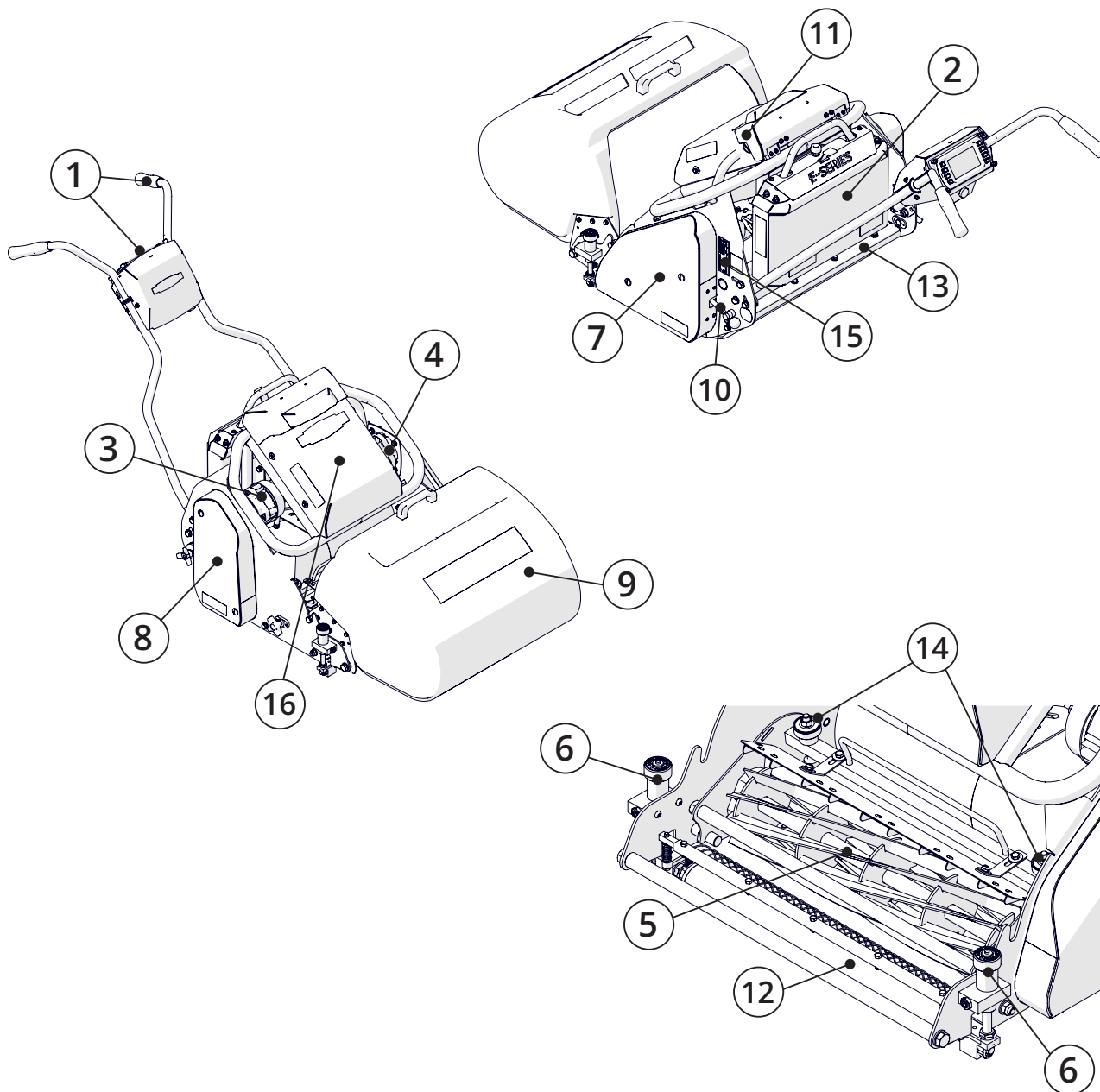
Fig.4. Machine components overview
