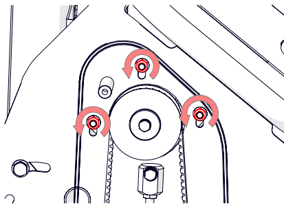
Fig. 19B - Loosen slightly the motor 3 x top nuts.
