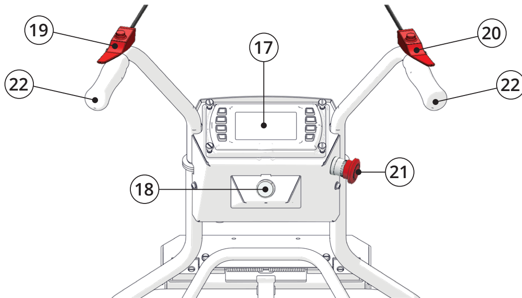
Fig.6. Control components overview
