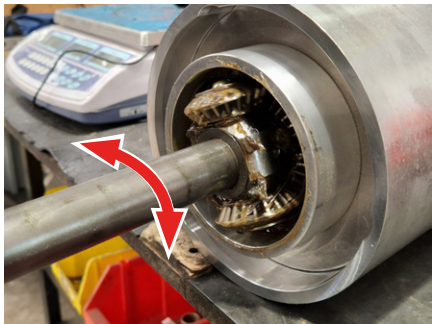
Fig. 25P - Rotate shaft to ensure grease is evenly distributed.
