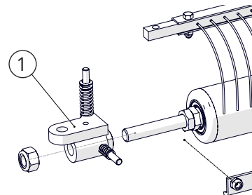
Fig. 27C - Remove comb tine and scraper to gain access to end block (1).
