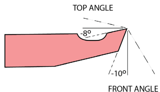
Fig.22. Recommended shear blade grind angle
