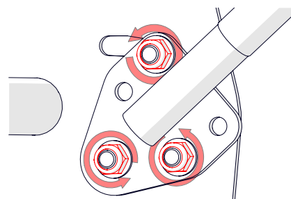
Fig.11B - Loosening the inner nut
