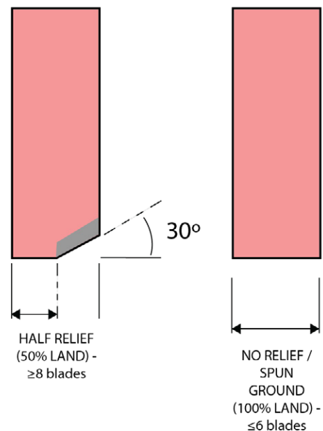
Fig.21. Recommended cylinder grind angle
