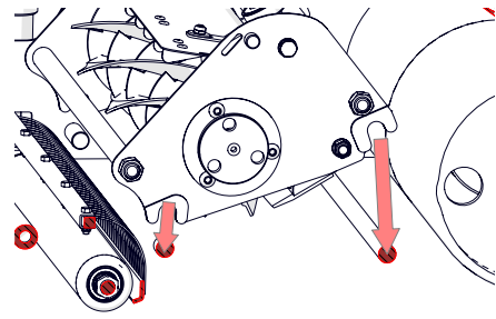
Fig.8E - Lower cassette onto tie-bars (cut-through).
