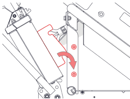
Fig. 17F - Cross section view of battery insertion - step 1.
