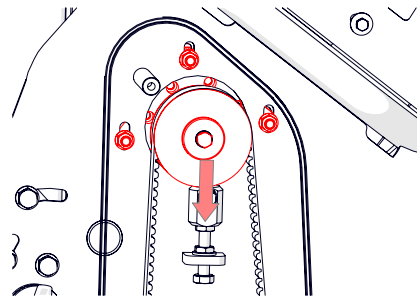
Fig. 19E - Support the weight and lower.
