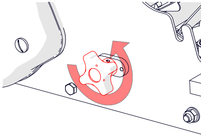
Fig.8A - Lower support stand
