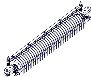
Fig. 27B - Whole front roller assembly.
