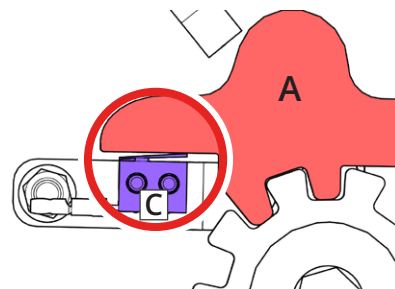
Fig. 24B - End of the brake hammer (A) presses the microswitch (C).
