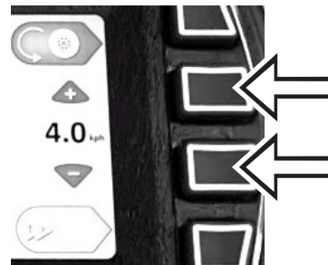
Fig.16. Adjusting Drive Speed
