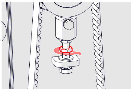
Fig. 19D - Loosen fully the tensioner block locking nut.
