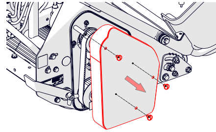
Fig. 25A - Remove 3 x outer screws and cover.
