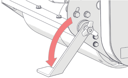
Fig.8A - Lower support stand
