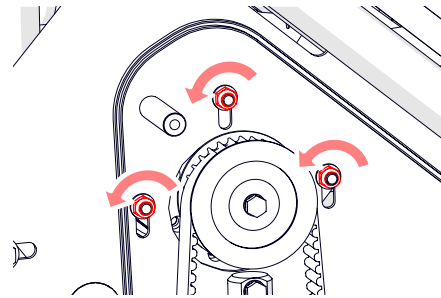
Fig. 25B - Loosen slightly the motor 3 x top nuts.
