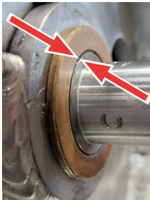
Fig. 25Q - Check for no lip between Oilite bush and shaft.
