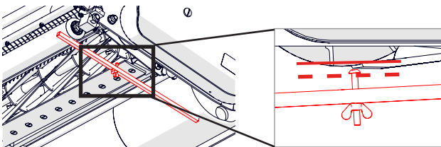
Fig. 9C - Position the setting bar and observe distance between the top of the shear blade and bottom on the bolt head. In this example, the underside of the bolt head is below (dashed line) the shear blade (solid line), indicating the machine cut height is currently too high and therefore needs lowering.
