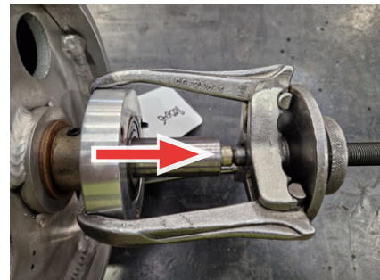
Fig. 25M - Remove the bearing.
