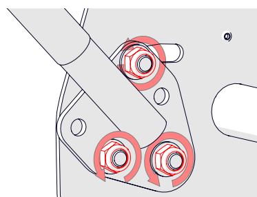
Fig.11C - Repeating adjustment for other side
