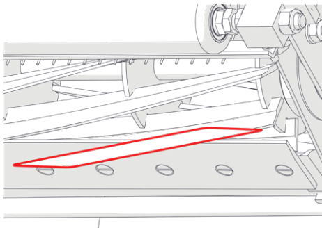
Fig.13B - Repeating adjustment for other side
