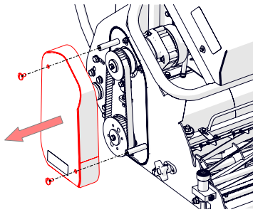
Fig. 19A - Remove 3 x outer screws and cover.
