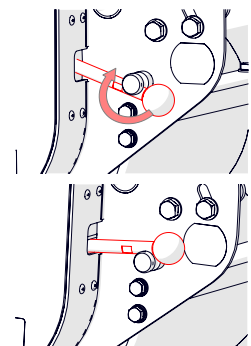
Fig.4A - Parking brake disengaged (top), and engaged (bottom).
