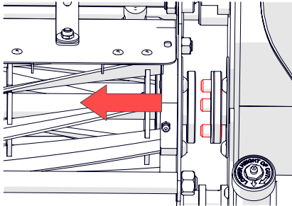
Fig.8C - Slide cassette until pins are visible.
