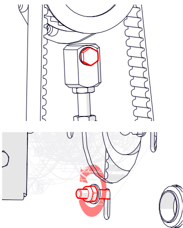
Fig. 19C - Loosen slightly the tensioner block/motor nut.
