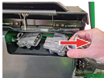
Fig. 17B - Disconnect the electrical connector.
