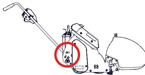
Fig.11A - Securing the bolt head
