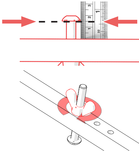
Fig.9A - Adjust bolt to desired cut height and secure nut (above example set for 15mm).
