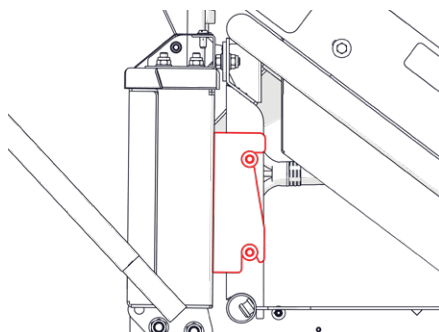
Fig. 17H - Cross section view of battery insertion - step 3.
