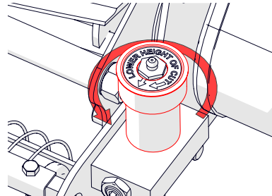
Fig. 27A - Loosen height adjusters.
