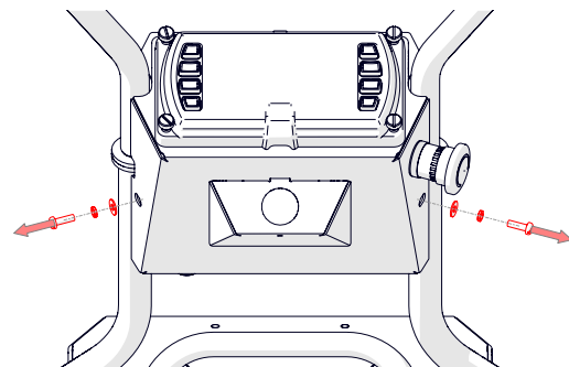
Fig.12D - Remove bottom console screws.
