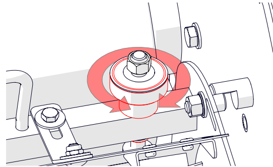
Fig.13D - Tighten/loosen the adjustment nut
