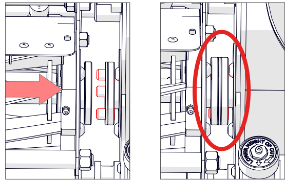
Fig.8F - Lower the new cassette in and slide across, engaging with three pins.
