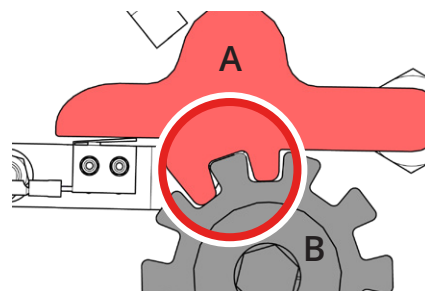
Fig. 24A - Brake hammer (A) engaging correctly with the cut-outs of the brake disc (B).
