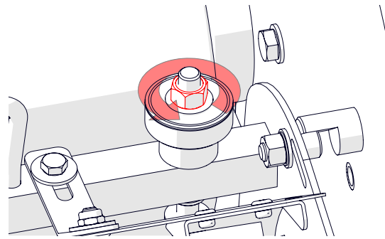
Fig.13C - Loosen the lock nut
