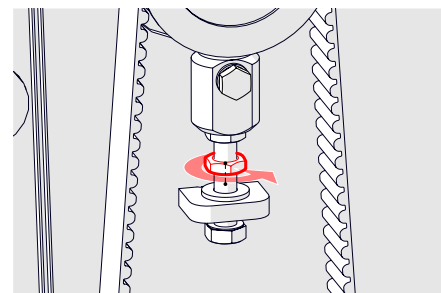
Fig. 25D - Loosen fully the tensioner block locking nut.
