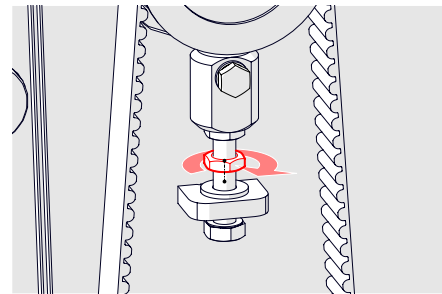
Fig. 19G - Tighten the belt and tensioner block locking nut.
